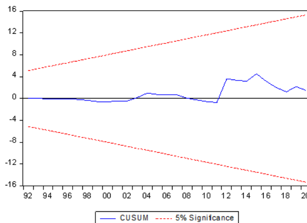
Figure 1 CUSUM square test
