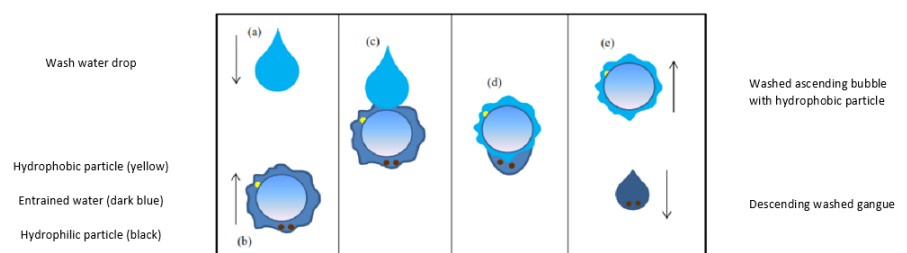
Figure 8 The froth washing mechanisms (a) drop of water descending into the froth, (b) mineral-laden air bubble rising in the froth with associated entrained water and particles (c) contact between the wash water and the air bubble, (d) the descending droplet of water displaces the entrained water and particles and, (e) entrained particles flow back into the pulp while the bubble with clean water ascends [66].
