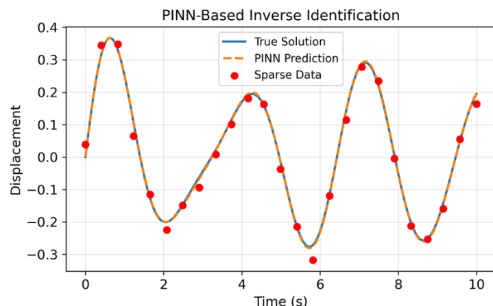
Figure 5 Comparison between the reference system response, the physics-informed digital twin (PINN) prediction, and the sparse noisy displacement measurements used for training. Despite being trained on limited and noisy data, the PINN accurately reconstructs the underlying system dynamics, capturing both the oscillatory behavior and amplitude decay. The predicted system remains smooth and physically consistent across the entire time domain, including regions between measurement points. This demonstrates the ability of the physics-informed framework to perform.
